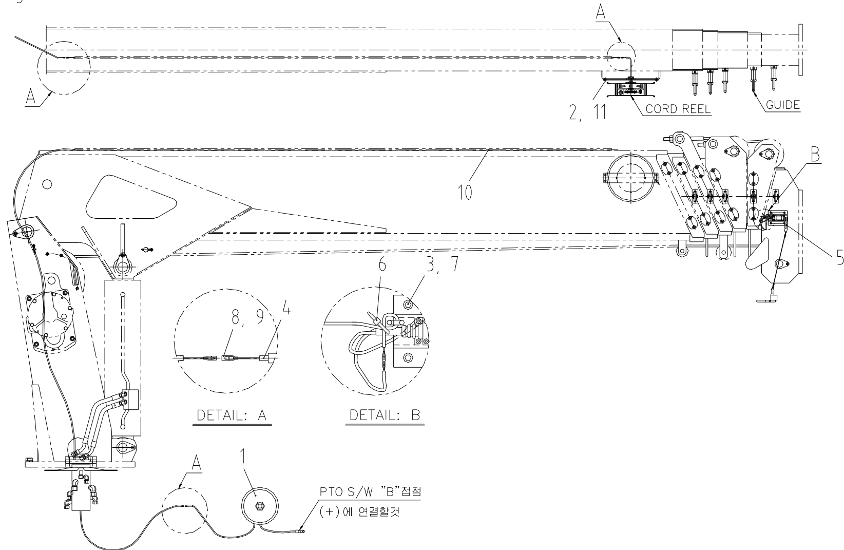
Fig. 9 SCS747L OVERWINDING ALARM DEVICE ASS'Y
