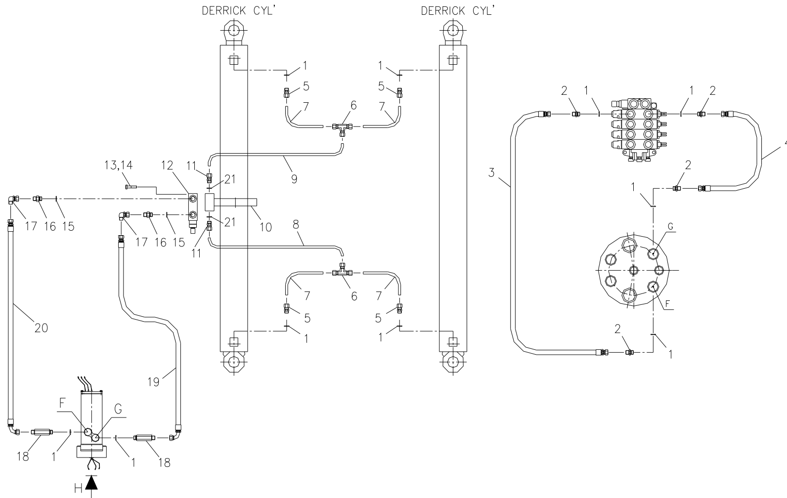
Fig. 5-2 SCS747L DERRICK PIPING
