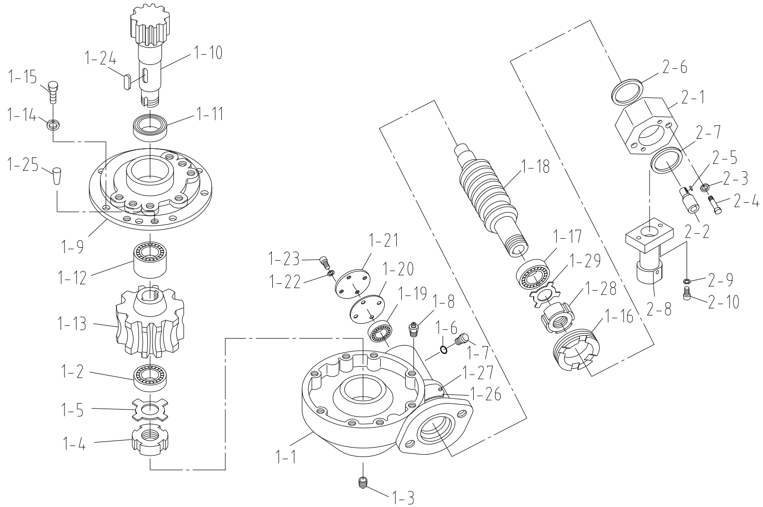
Fig. 3-1 SCS747L SWING R/G ASS'Y
