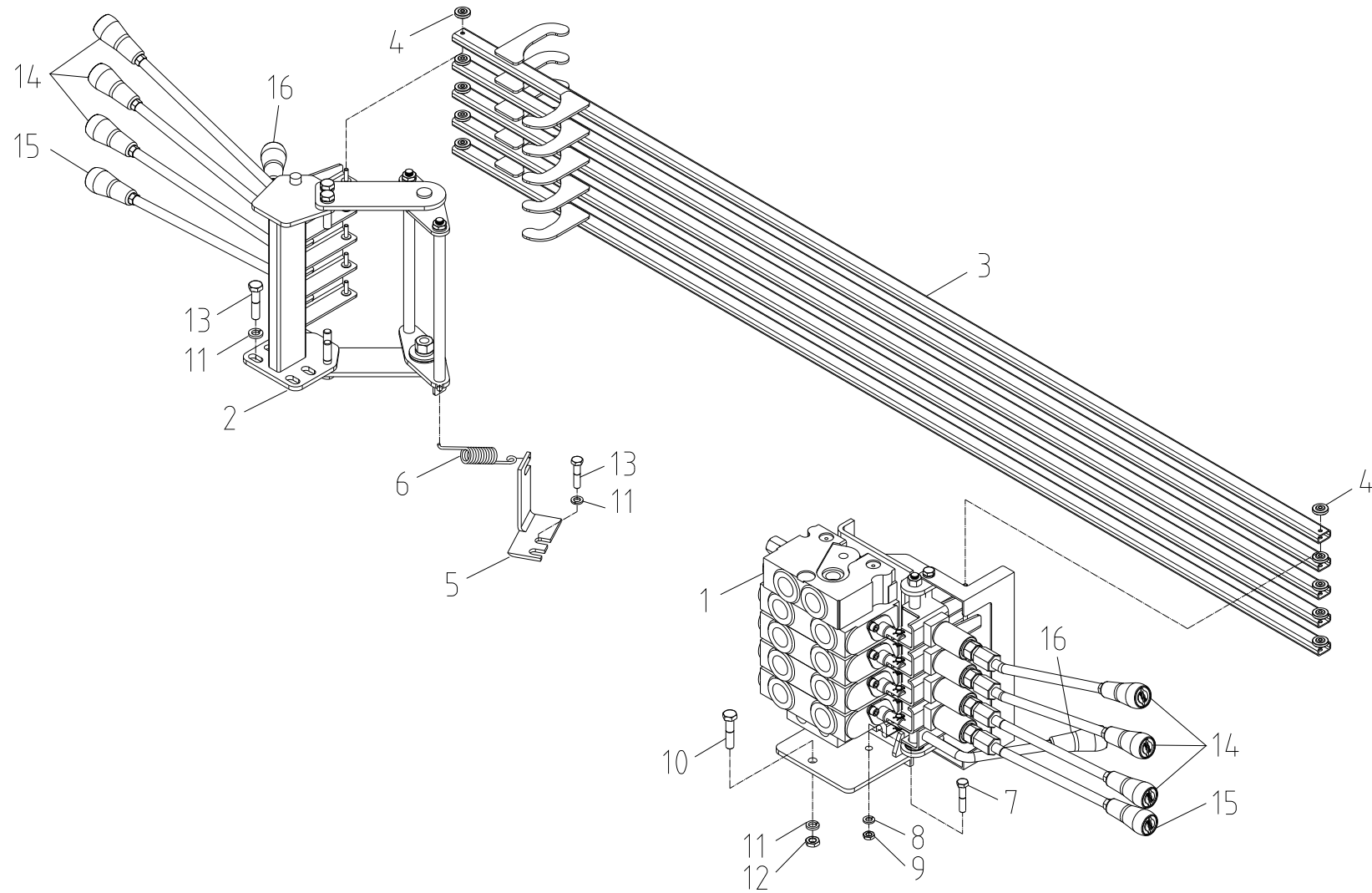
Fig. 3-3 SCS747L OPERATION MAIN ASS'Y
