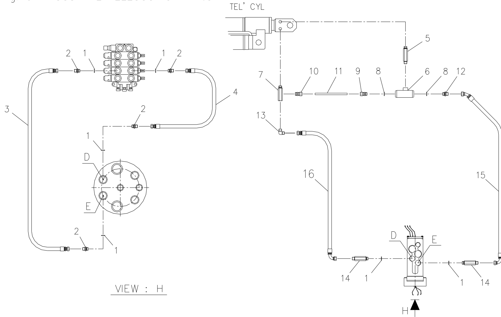
Fig. 5-4 SCS747L TELESCOPIC PIPING
