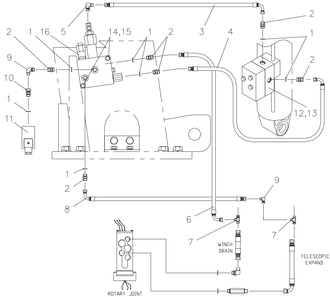
Fig. 5-7 SCS747L LOAD LIMMIT PIPING
