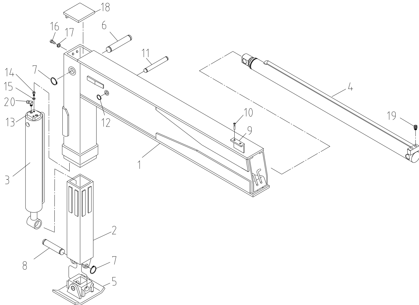
Fig. 4 SCS747L OUTRIGGER ASS'Y(5TON)
